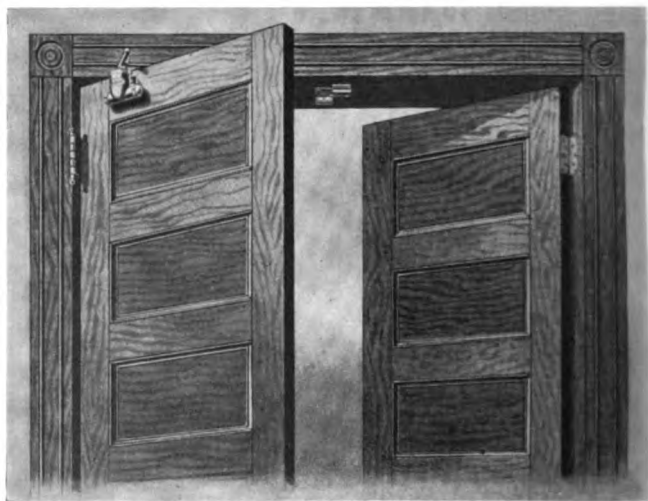
Fig. 4. The Yale-Blount Check and Duplex Stop.
