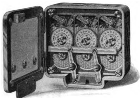
Fig. 1. Yale Time-lock with 3 Chronometer Movements.
