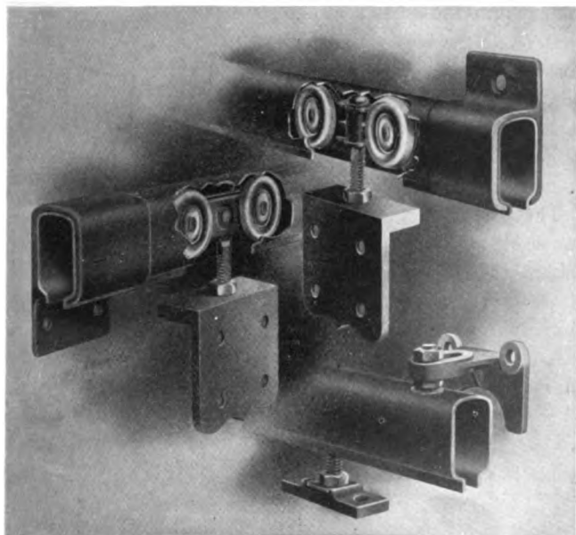
Fig. 4. Steel Hangers and Tracks.
