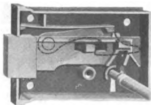
Fig. 9. Warded Lock.
