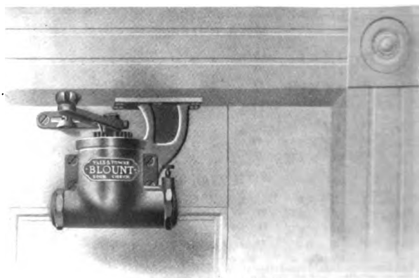
Fig. 2. Right-hand Door From Outside. Use Left-hand Check with Bracket.
