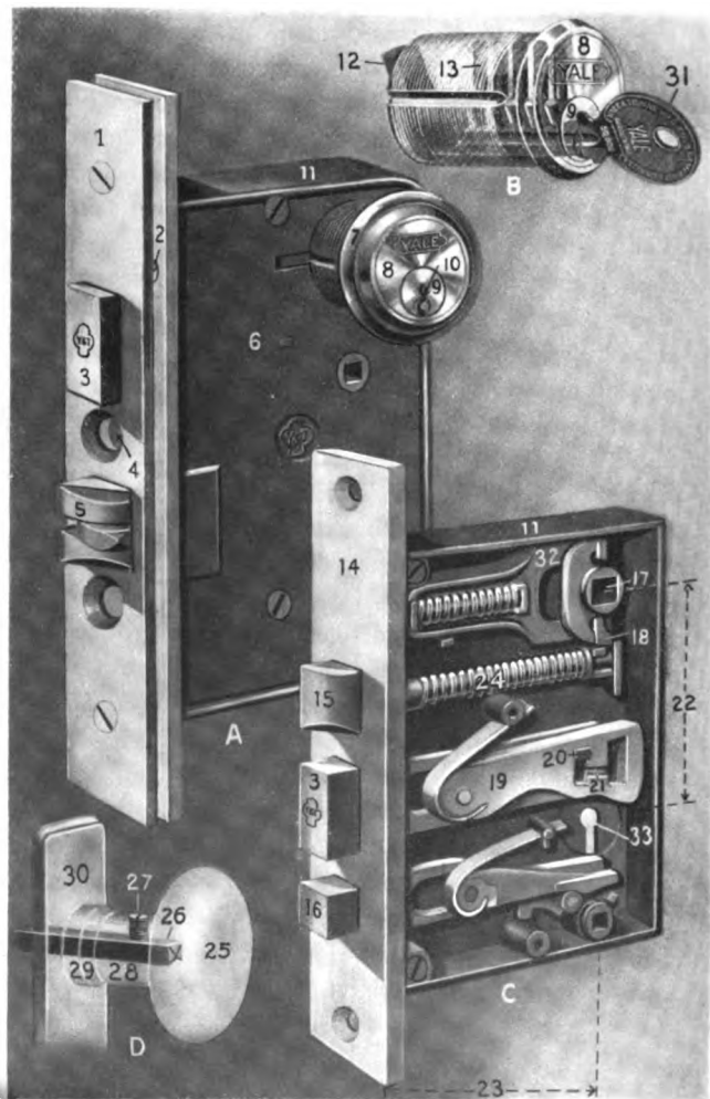
Builders' Locks and their Details.
