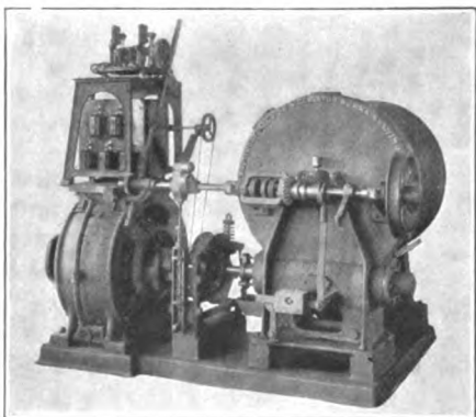
Type S Motor Driving Elevator Hoist
